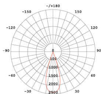
36° fascio/beam 2700°K
