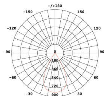
60° fascio/beam
