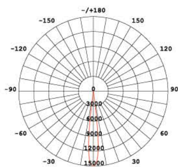
15° fascio/beam
