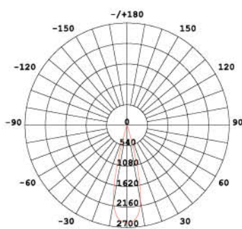
25° fascio/beam
