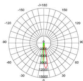
12° fascio/beam
