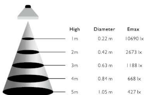
12° fascio/beam
