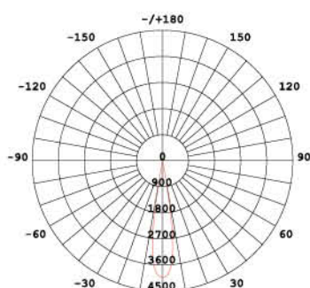
15° fascio/beam
