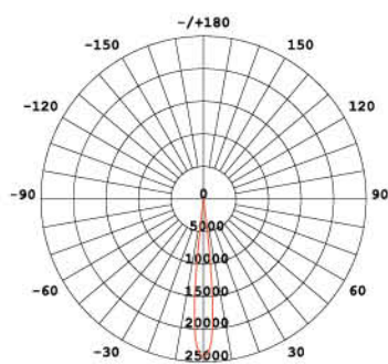
10° fascio/beam
