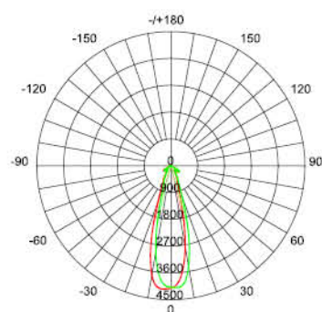
30° fascio/beam
