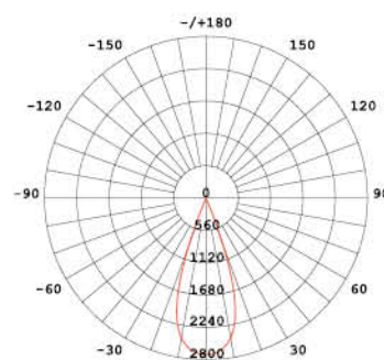
36° fascio/beam 4000°K
