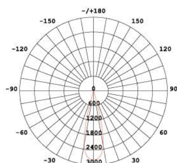
25° fascio/beam
