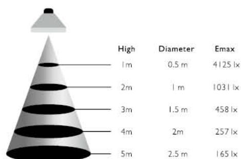
30° fascio/beam
