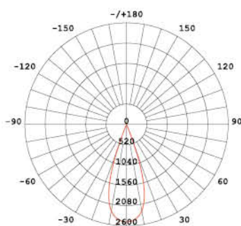
36° fascio/beam 3000°K
